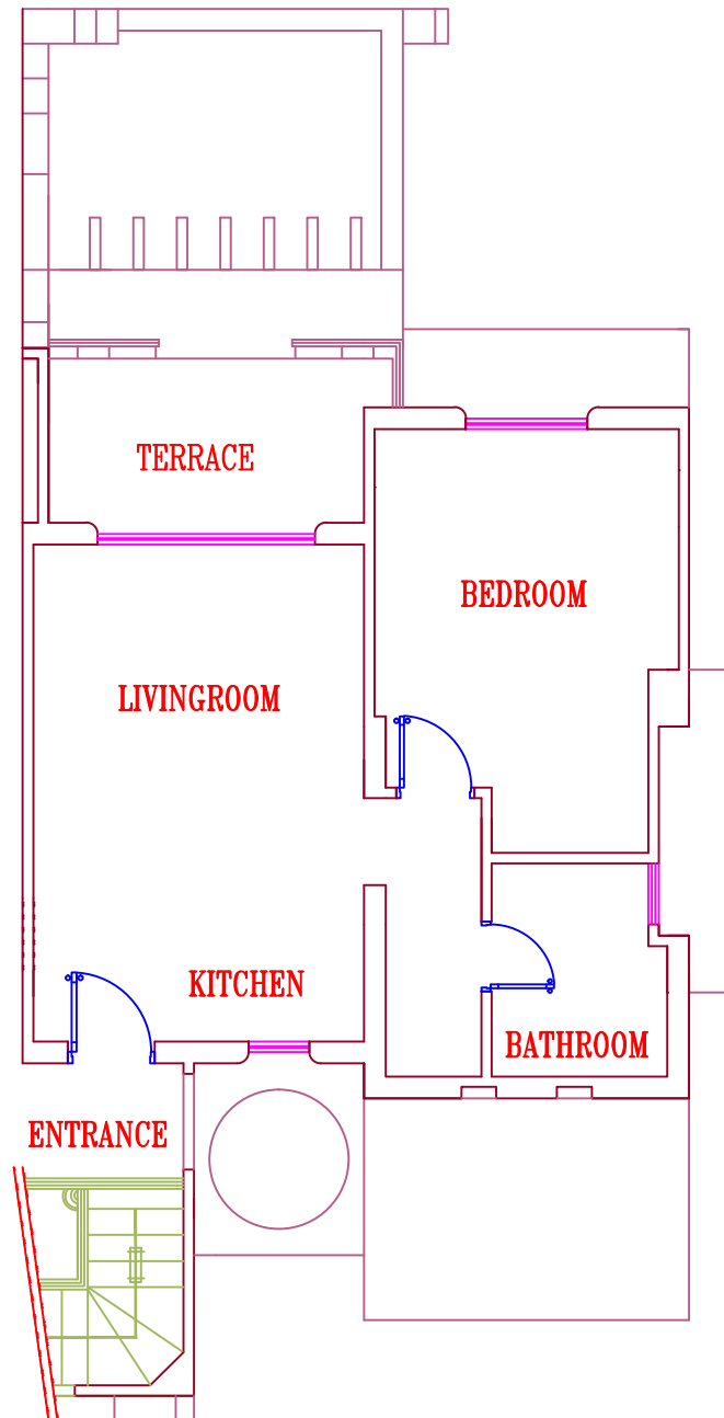
SECOND FLOOR PLAN CHALET
